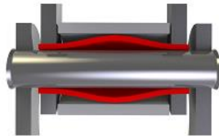
Picture 2: The difference between ČZ KSJ bushes and standard ČZ bushes
